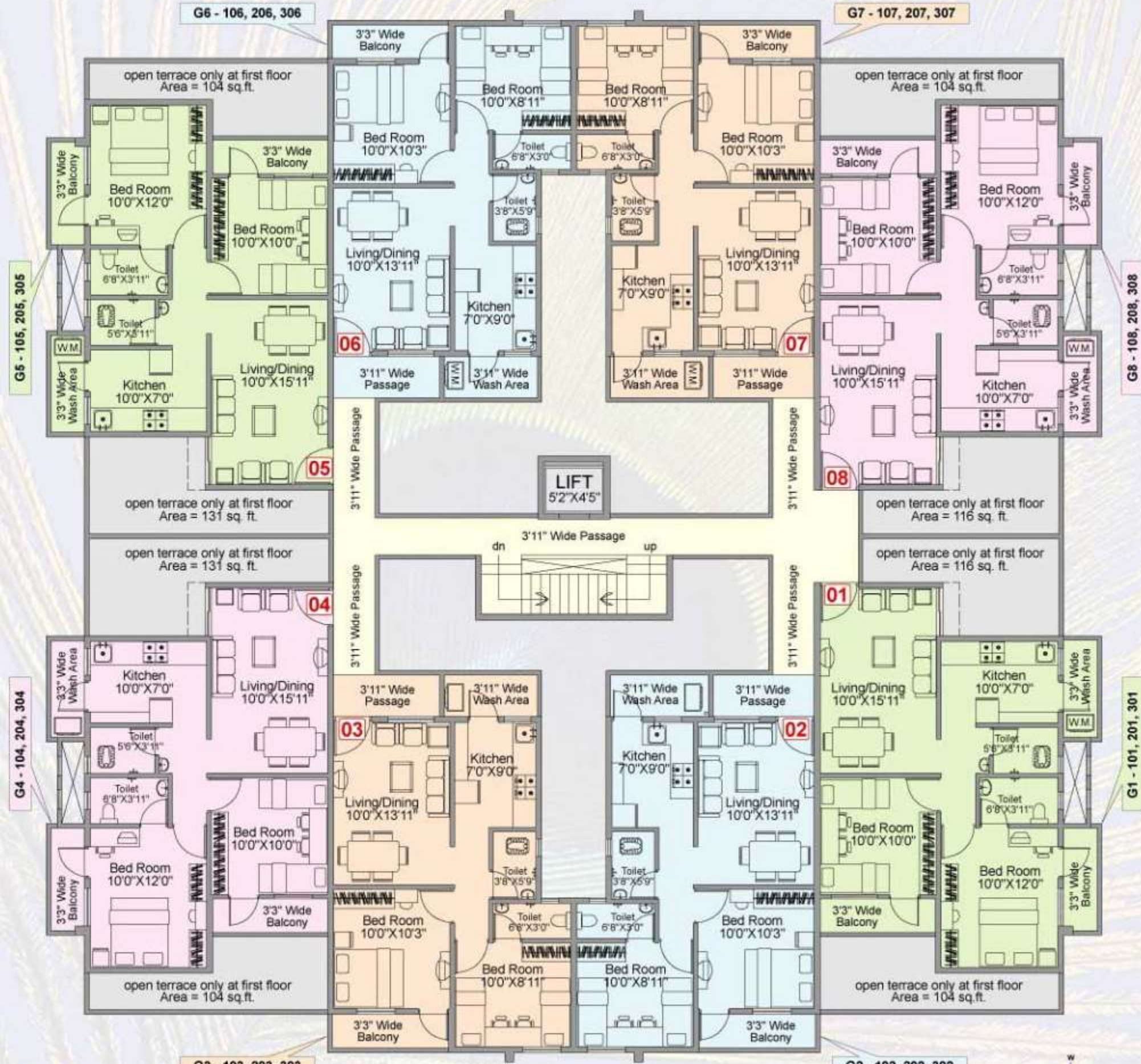
Ground Floor To Third Floor Plan
